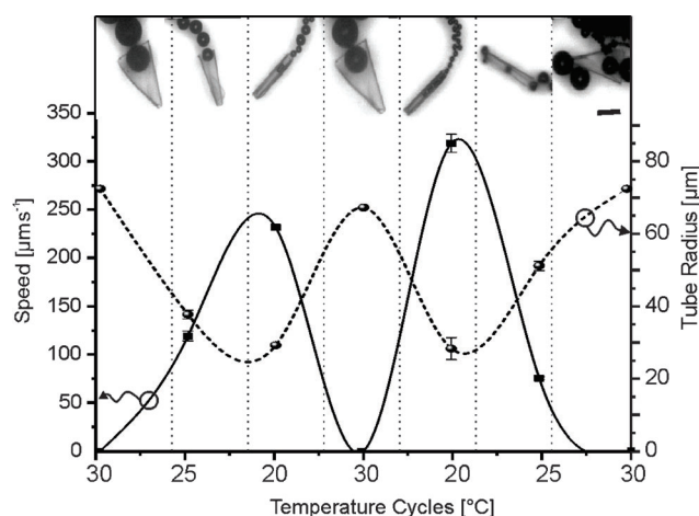
Figure 4. Cycles of folding and unfolding of thermoresponsive 265 \mu\text{m} -long polymer-Pt jets in 5 wt% H 2 O 2 solution with 0.1% Triton X as surfactant by cooling below and heating above 28 ^\circ\text{C} . The graph plots the average speed [ \mu\text{m s}^{-1} ] (left y-axis, continuous line) and tube radius [ \mu\text{m} ] (right y-axis, dotted line) of polymer-Pt-microjets over the temperature cycles. Insets: snapshots of Pt-polymer jets with changing radius owing to the compressing at temperatures below 28 ^\circ\text{C} and expanding at temperatures above 28 ^\circ\text{C} . Scale bar: 100 \mu\text{m} (Supporting Information, Videos S4a and S4b). Error bars: standard deviation for n = 3 .
